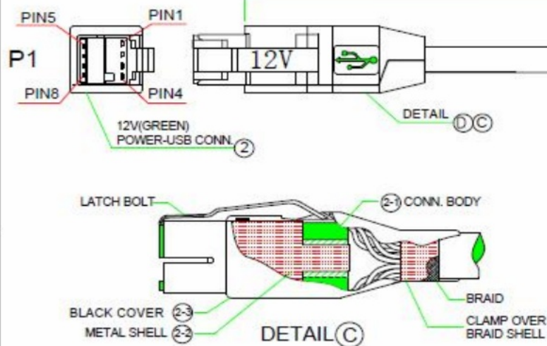
WIRE LIST
