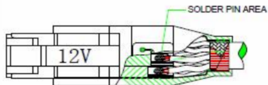
DETAIL D
